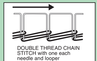
PLAIN SEWN CLOSURE
